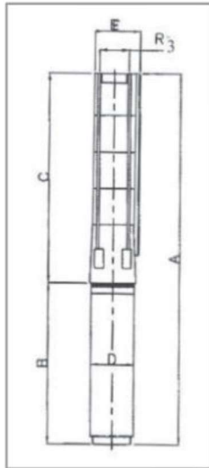
LB 30 - 39 to LB 30-54 pumps are mounted in S.S. Sleeve.
